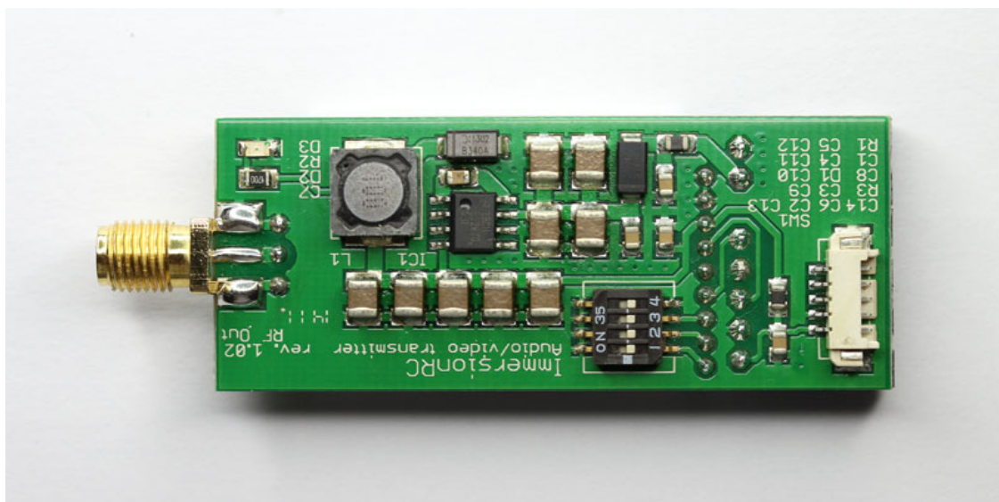
Fig 2. Bottom side of ImmersionRC 700mW 2.4GHz audio/video transmitter.
